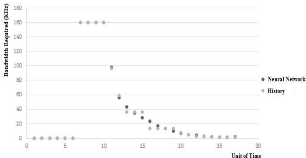
Fig. 7 Predicted exponential distribution for variable BW
