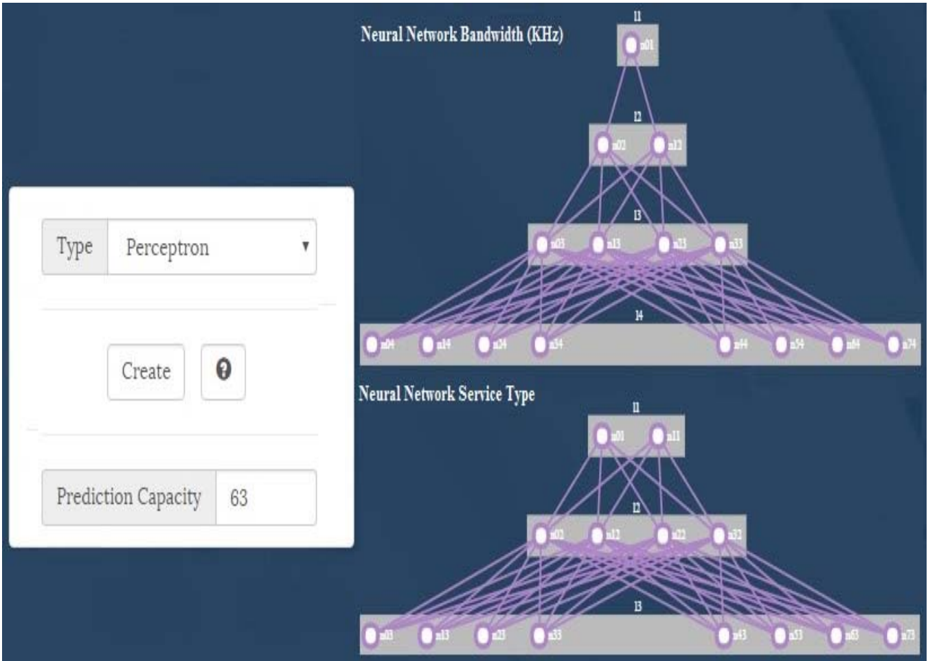
Fig. 4 Creation stage of the specialized MLPNNs
