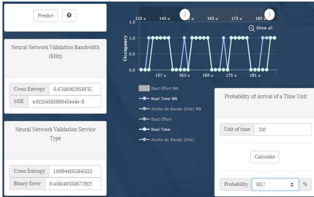
Fig. 6 Prediction phase (probability calculation of a QoS request) of the neural network
