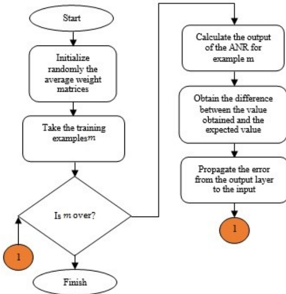
Fig. 2 MLPNN Training Diagram
