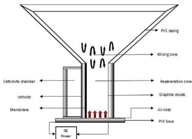
Fig. 1 Sequential batch electrochemical cell used for electrochemical regeneration of Nyex 100 and composite adsorbent
