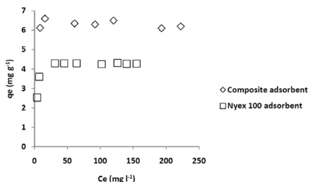
Fig. 3 Adsorption isotherms for acid violet 17 onto Nyex 100 in a 250 ml flask using a contact time of 60 minutes
