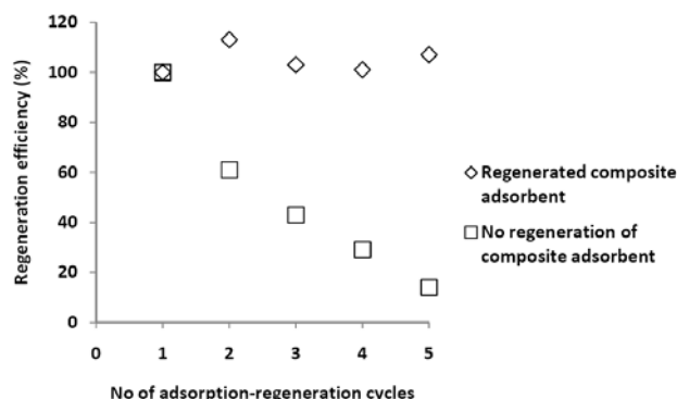
Fig. 5 Electrochemical regeneration efficiency (based on colour removal) for a number of adsorption-regeneration cycles with acid violet 17 / composite adsorbent using a sequential batch cell. Operating parameters; Current 1 A and treatment time 60 min
