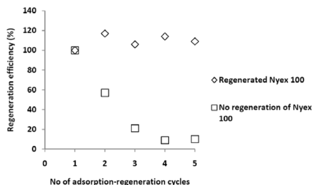
Fig. 4 Electrochemical regeneration efficiency (based on colour removal) for a number of adsorption-regeneration cycles with acid violet 17 / Nyex 100 using sequential batch cell. Operating parameters; Current 1 A and treatment time 60 min
