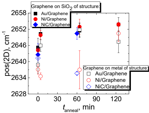
Fig. 8 Raman shift of 2D peak position versus anneal time: solid symbol represents graphene on SiO 2 (between Au (black), Ni (red) and NiC (blue) metal contacts). Unfilled symbol represents Au/Graphene (black), Ni/Graphene (red) and NiC/Graphene (blue) metal contacts
