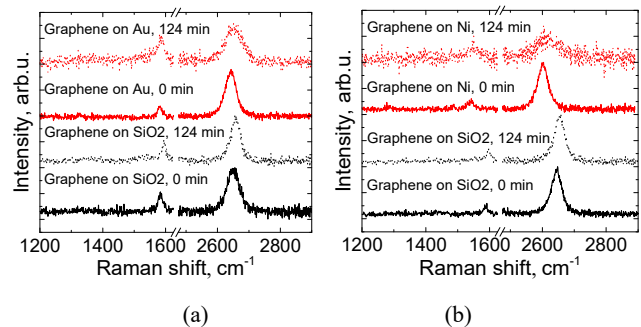
Fig. 7 Raman spectra of graphene transferred on \text{SiO}_2 substrate and metal contacts before annealing (solid line) and after 2h annealing (dots); (a) Raman spectra of graphene transferred on \text{SiO}_2 substrate and Au contacts (b) Raman spectra of graphene transferred on \text{SiO}_2 substrate and Ni contacts
