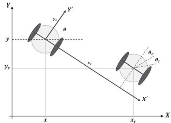
Fig. 1 Mobile robot in X-Y coordination
