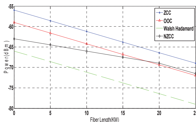
Fig. 5 Received Power (dBm) vs Fiber length for various codes in SAC-OCDMA technique
