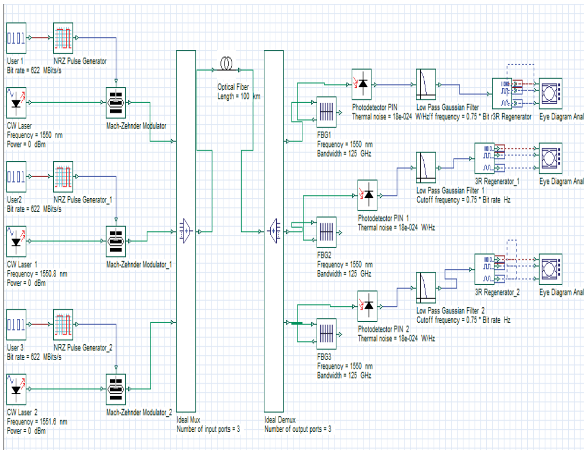
Fig. 2 Simulation circuit for 3 users [19]
