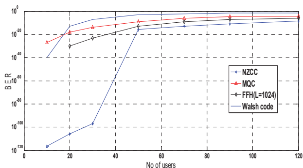
Fig. 3 BER vs. No of users for various codes at 1 Gbps data rate in SAC-OCDMA technique
