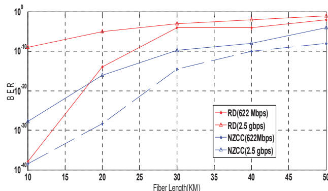
Fig. 4 BER vs Fiber length for various codes employing different data rates in SAC-OCDMA technique
