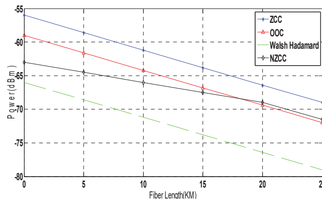
Fig. 5 Received Power (dBm) vs Fiber length for various codes in SAC-OCDMA technique
