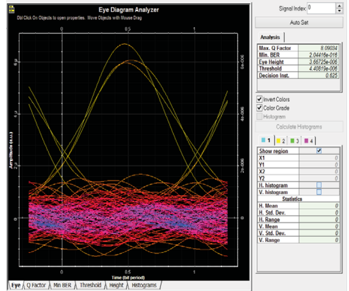
Fig. 9 Eye diagram indicating performance of 50 user, -10 dBm power, 50 km length for NZCC code
