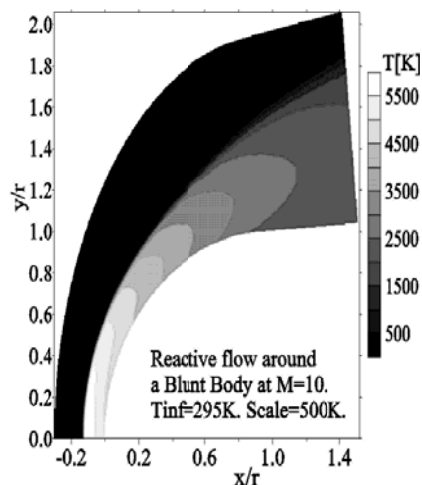
Fig. 12 Temperature contours
