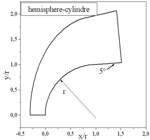
Fig. 4 Computational domain
