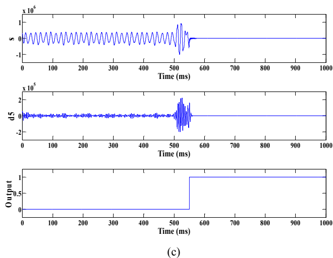
Fig. 6 Ferroresonance detection for IEDs using proposed algorithm
