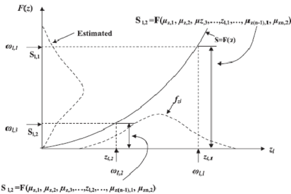
Fig. 1 Conceptual illustration of the 2m PEM
