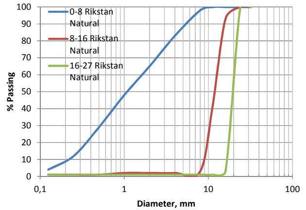
Fig. 1 Sieve curves showing the 0-8 mm, 8-16 mm and 16-27 mm fractions for the natural Riksten material.
