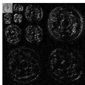
Fig. 2 Tree level wavelet decomposition
