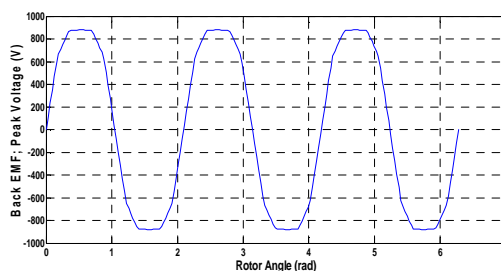
Fig. 20 Initial EMF Waveform
