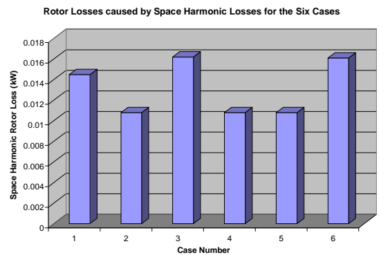
Fig. 40 Rotor Loss Caused by Space Harmonics Comparisons
