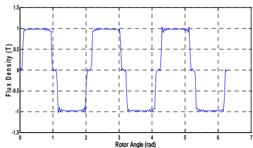
Fig. 16 Initial Flux Density Waveform
