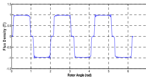
Fig. 19 Initial Flux Density Waveform
