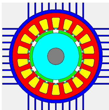
Fig.2 Surface mounted PM machine shape.
