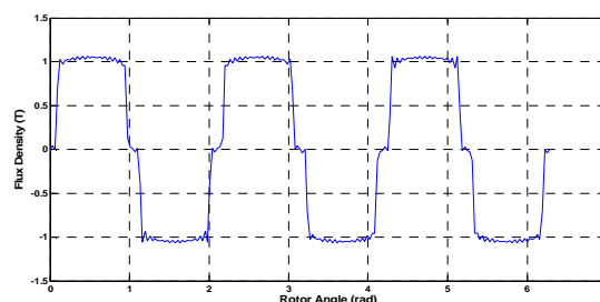
Fig. 22 Initial Flux Density Waveform
