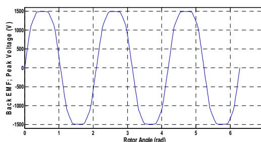
Fig. 23 Initial Back EMF Waveform
