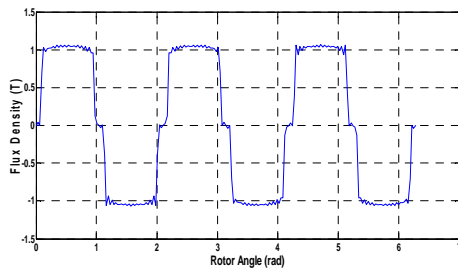
Fig. 14 Initial EMF Waveform
