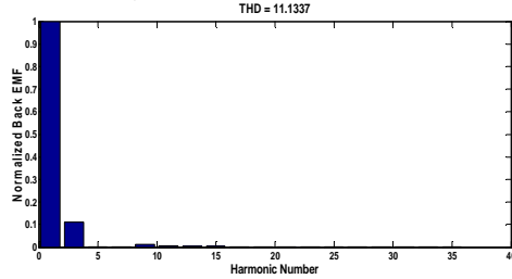
Fig. 15 Initial Harmonic Content (11.1337 %) for case 3
