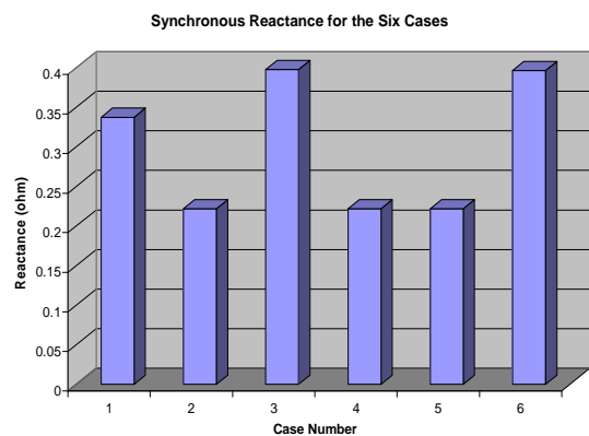
Fig. 32 Synchronous Reactance Comparisons
