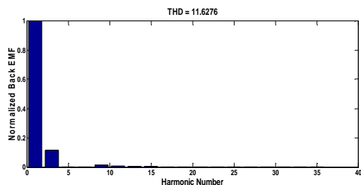
Fig. 21 Initial Harmonic Content (11.6276 %) for case 5
