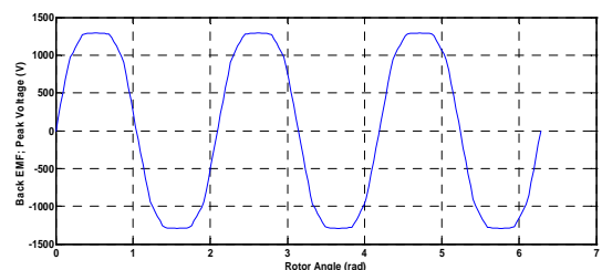
Fig. 8 Initial EMF Waveform
