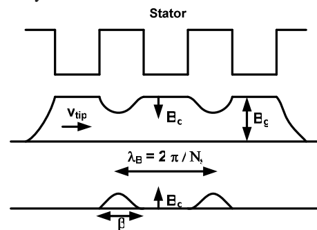
Fig. 6 Flux Density Variation
