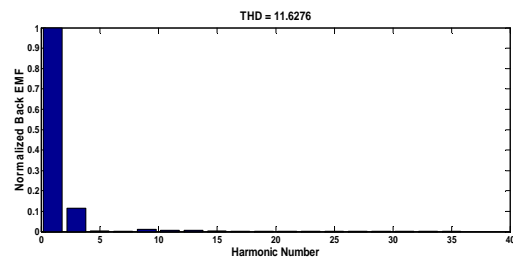
Fig. 12 Initial Harmonic Content (11.6276 %) for case 2
