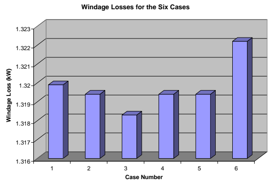
Fig. 37 Windage Loss Comparisons
