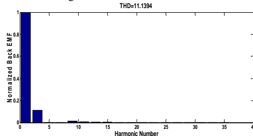
Fig. 24 Initial Harmonic Content (11.1394 %) for case 6
