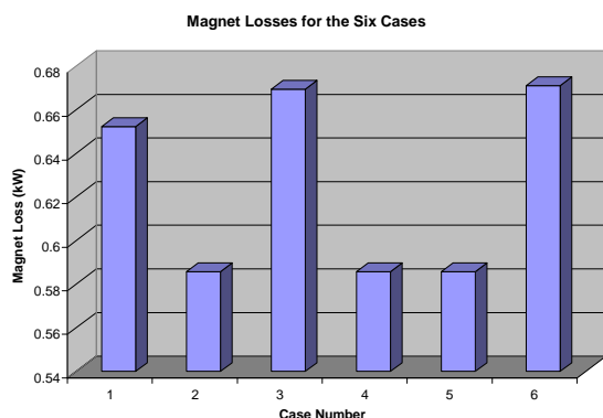
Fig. 41 Magnet Loss Comparisons
