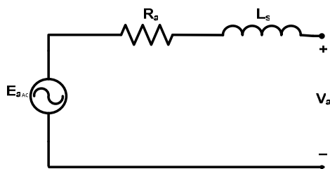
Fig. 3 A Per Phase electrical model.
