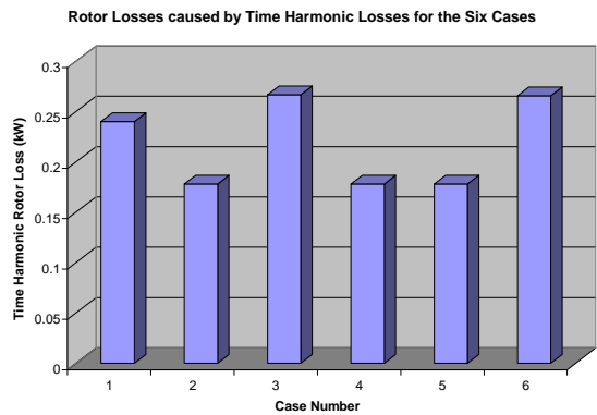
Fig. 39 Rotor Loss Caused by Time Harmonics Comparisons
