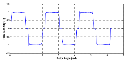
Fig. 11 Initial EMF Waveform
