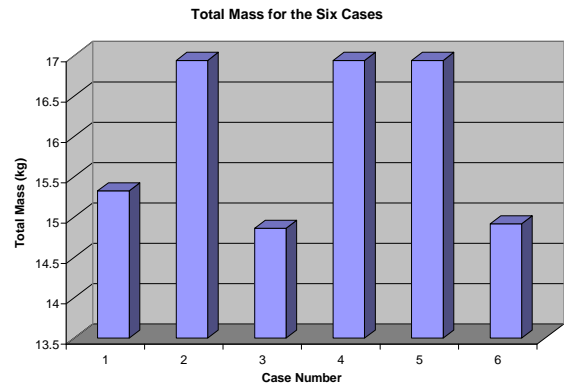
Fig. 38 Total Mass Comparisons
