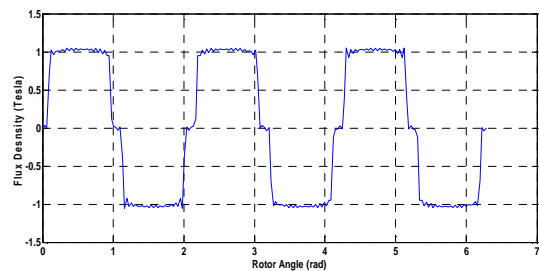
Fig. 7 Initial Flux Density Waveform
