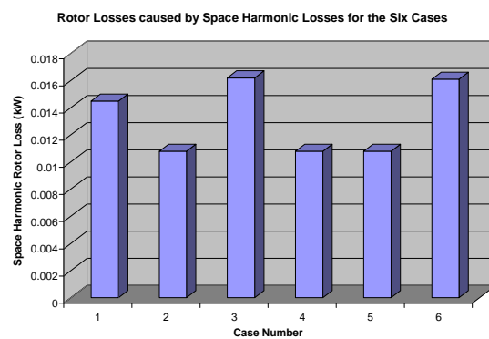
Fig. 40 Rotor Loss Caused by Space Harmonics Comparisons
