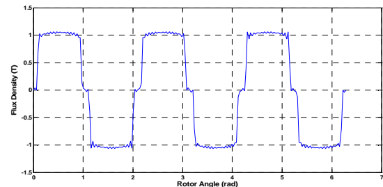
Fig. 22 Initial Flux Density Waveform
