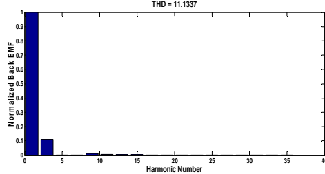
Fig. 15 Initial Harmonic Content (11.1337 %) for case 3
