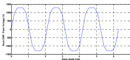
Fig. 8 Initial EMF Waveform
