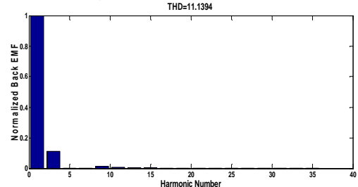
Fig. 24 Initial Harmonic Content (11.1394 %) for case 6
