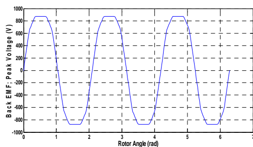
Fig. 17 Initial EMF Waveform
