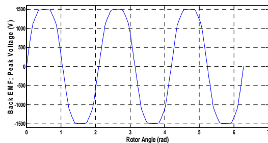
Fig. 23 Initial EMF Waveform
