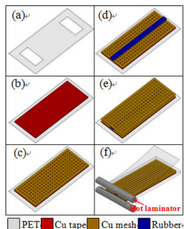
Fig. 2 Fabrication process of PET heat pipe
