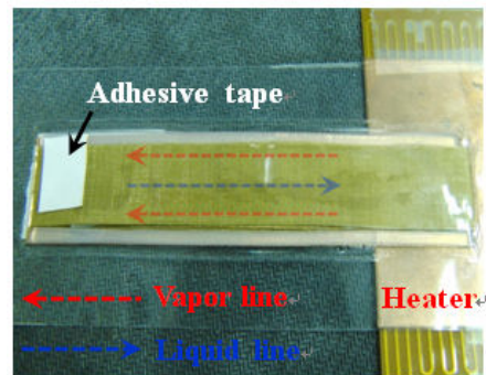
Fig. 11 Two-phase flow in PET heat pipe
