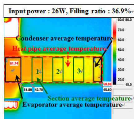
Fig. 7 IR thermal image for calculation the heat pipe average temperature
