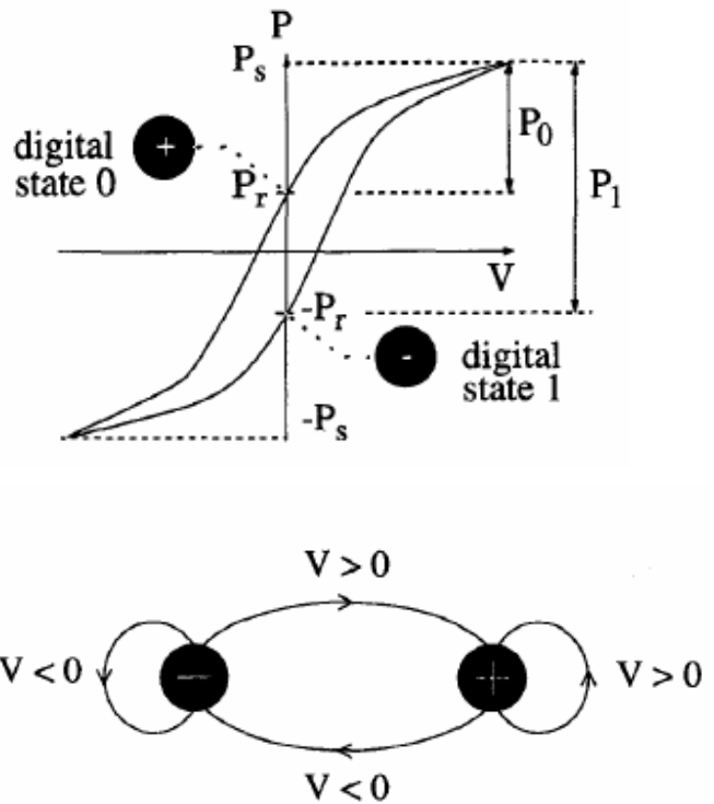
Fig. 4 State-wise Transition
