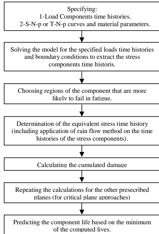
Fig. 4 The proposed numerical life assessment scheme
