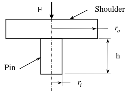
Fig. 2 Geometry of the FSW tool
