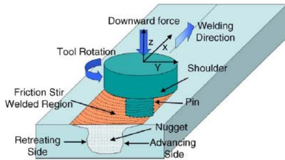
Fig. 1 A schematic of friction-stir welding process.
