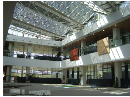
Fig. 6 Isofóton Headquarters, Malaga - Interior view of the atrium with elements with monocrystalline cell modules [3]
