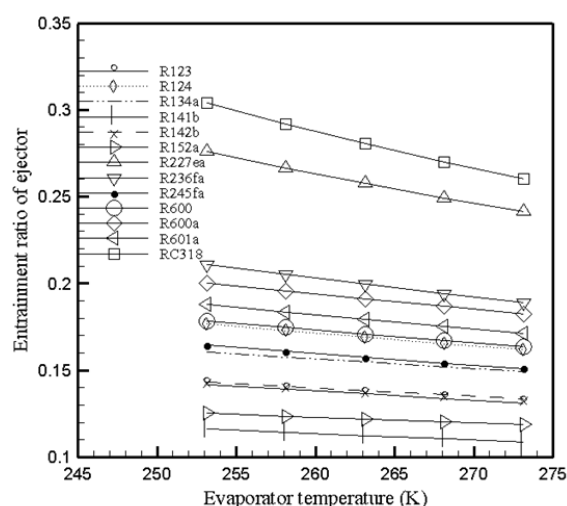
Fig. 3 Effect of the evaporator temperature on the entrainment ratio of ejector
