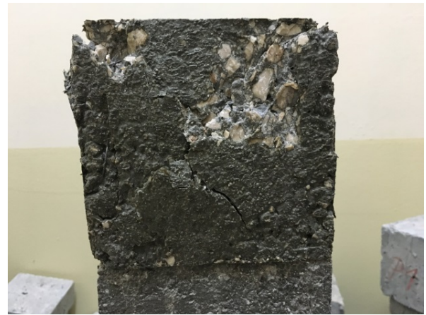
Fig. 3 Specimen after compressive strength test
