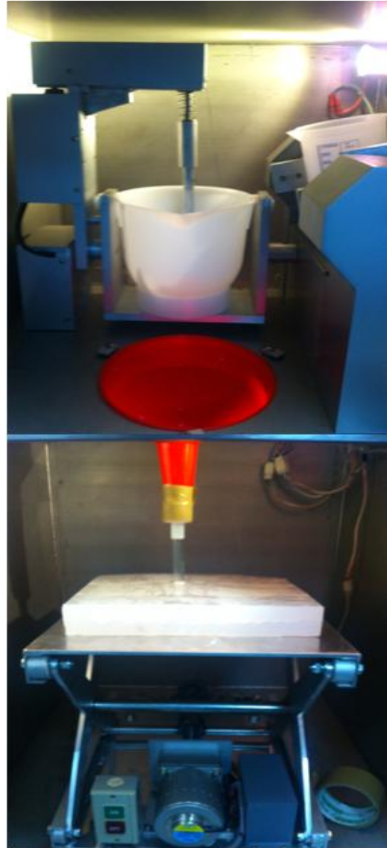
Fig. 3 Vacuum casting for fabricating the modeling platform
