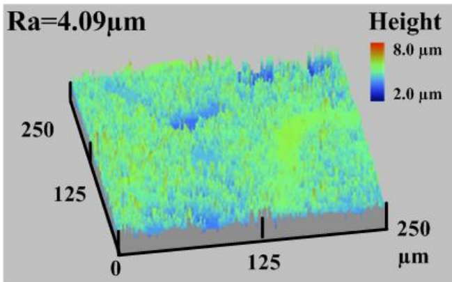
Fig. 10 Surface roughness of original modeling platform
