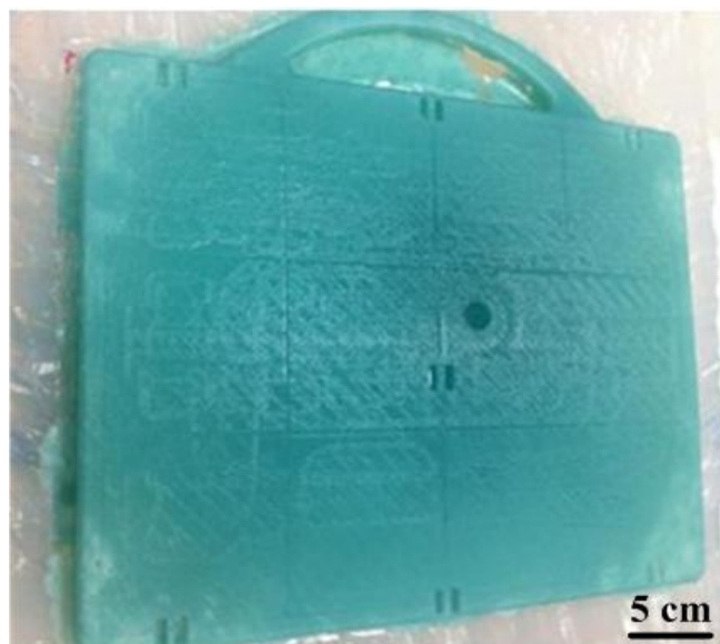
Fig. 5 Wax pattern of the modeling platform cast from silicone rubber mold
