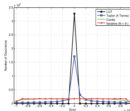
Fig. 11. Error distribution of efficient algorithms
