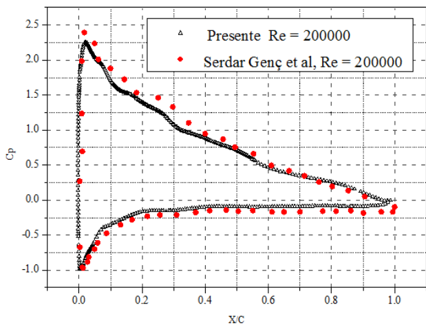
Fig. 3 Pressure coefficient
