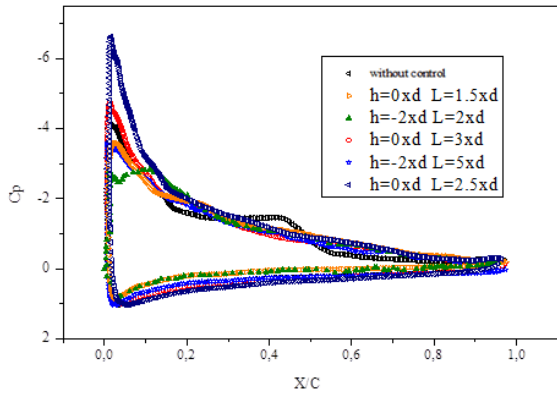
Fig. 7 Mean pressure coefficient
