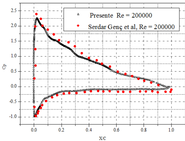
Fig. 3 Pressure coefficient
