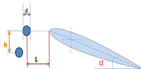
Fig. 1 Rod-foil geometrical characteristics
