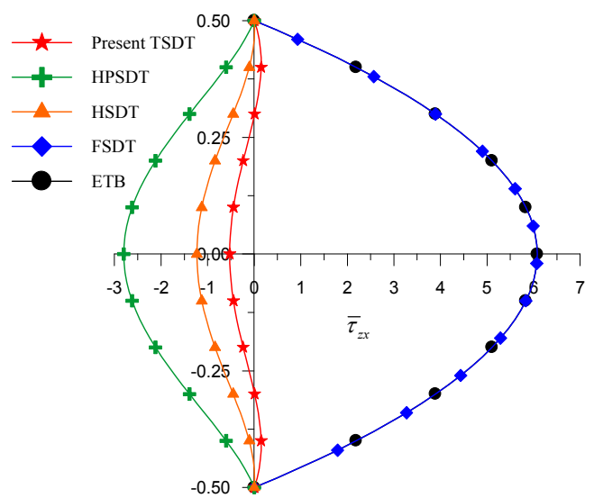
Fig. 11 Variation of transverse shear stress ( \bar{\tau}_{zx} ) through the thickness of simply supported beam at ( x = 0, z ) when subjected to cosine load and obtain using equilibrium equation for aspect ratio 10 (Example 1)
