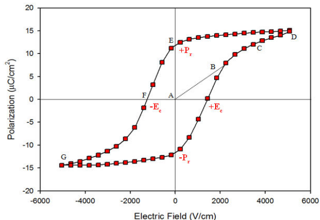
Fig. 2 Sample hysteresis loop of BaTiO 3 material
