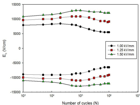
Fig. 10 Coercive field under difference electric field
