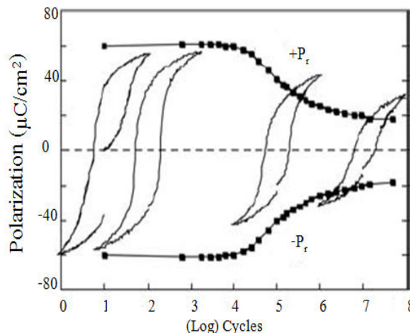
Fig. 3 Sample fatigue in PZT ceramic [8]
