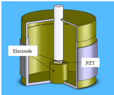
Fig. 5 Testing chamber
