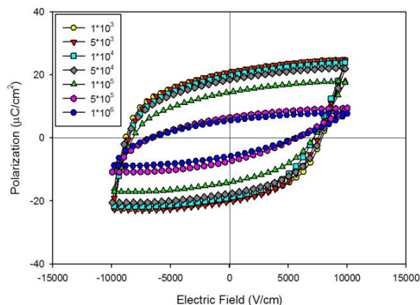
Fig. 6 Hysteresis loop with difference cycles (Electric field stress 1kV/mm)
