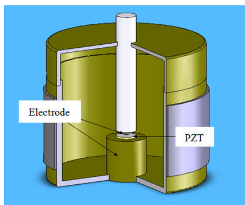
Fig. 5 Testing chamber
