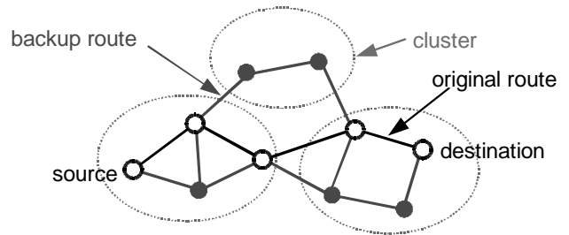
Fig. 5 New method A
