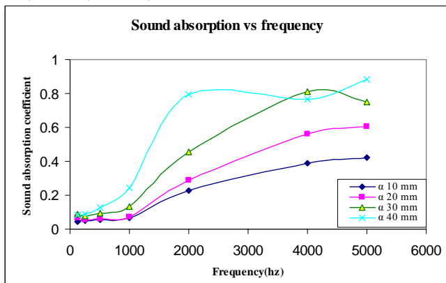
Fig. 2: Sound absorption of Arenga pinnata fiber
