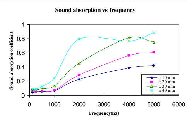
Fig. 2: Sound absorption of Arenga pinnata fiber
