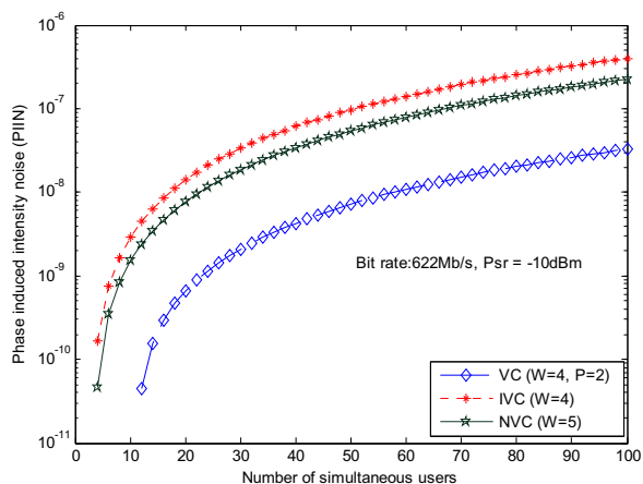
Fig. 8: PIIN Noise versus Number of Active Users for IVC, NVC and VC codes at data rate 622Mb/s when Psr = -10dBm.
