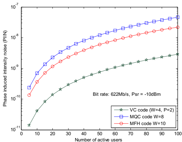
Fig. 9: PIIN Noise versus Number of Active Users for VC, MQC and MFH codes at data rate 622Mb/s when Psr = -10dBm.
