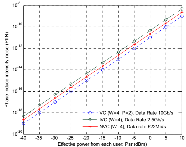
Fig. 6: PIIN Noise versus Received Power for IVC, NVC and VC codes at different data rates for W=4 .
