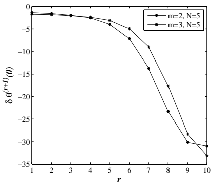
Fig. 9 Logarithmic graph of absolute \delta\theta ( \theta ) for m = 2, N = 5 and m = 3, N = 5(r+1)
