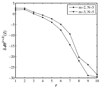
Fig. 10 Logarithmic graph of absolute \delta d\theta ( r+1 ) for m = 2, N = 5 and m = 3, N = 5
