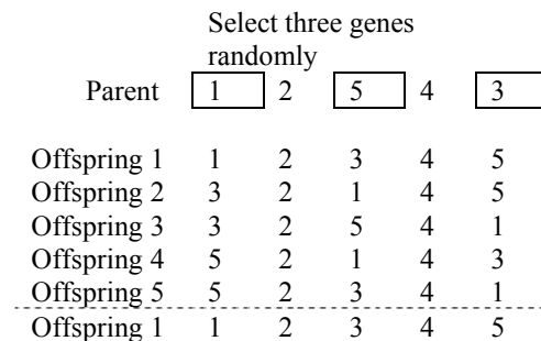
Fig. 4 The heuristic mutation operator
