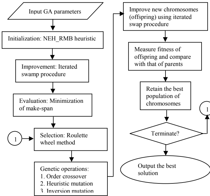
Fig. 1 The flowchart of the HGA
