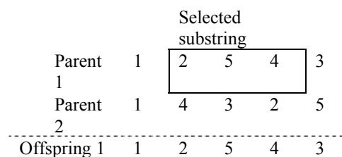
Fig. 3 The order crossover operator
