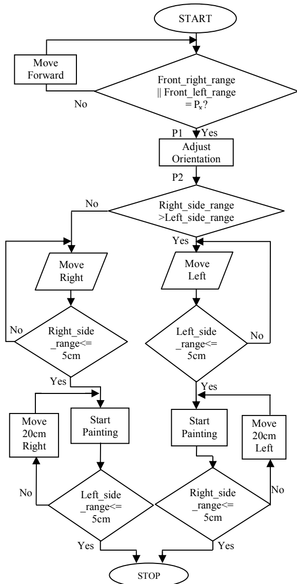
Fig. 12 Flowchart for control algorithm
