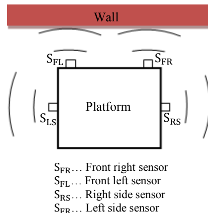
Fig. 11 Schematic representation of ultrasonic sensors as position and orientation feedback devices
