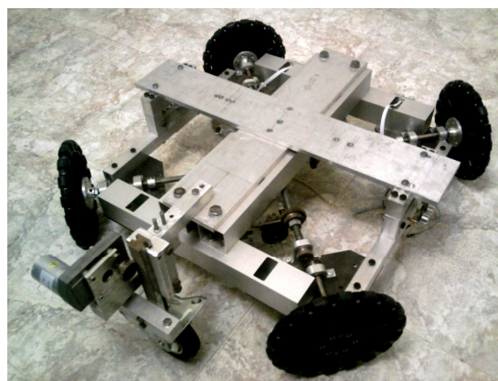
Fig. 17 Photograph of the mobile platform
