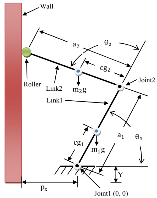
Fig. 1 Roller-based Wall Painting Robot in concept
