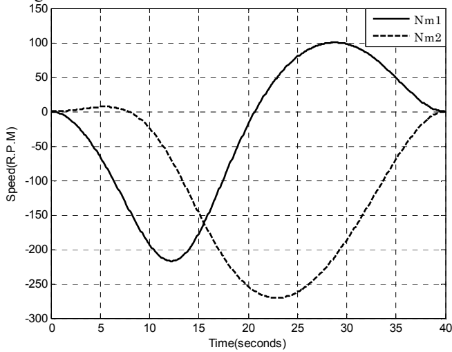
Fig. 6 Driving motors velocity profile
