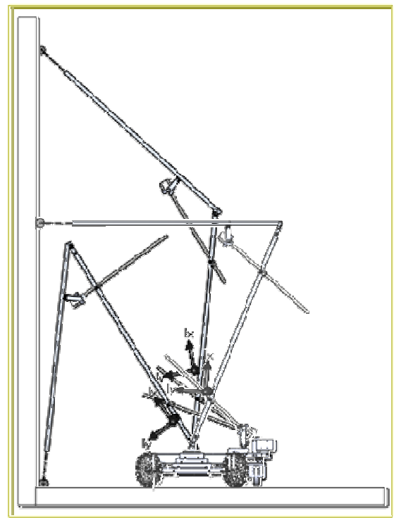
Fig. 9 C.G variation with the three extreme configurations
