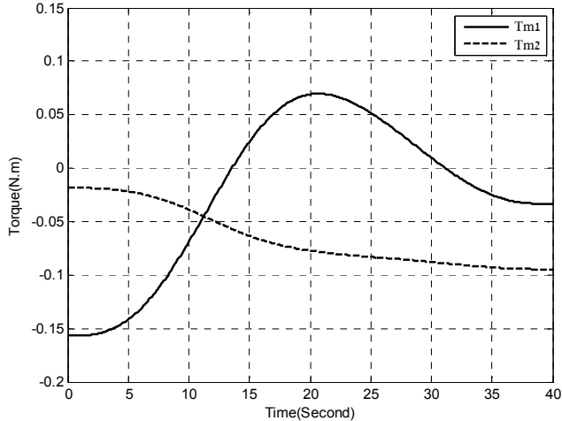
Fig. 7 Driving motors torque requirements
