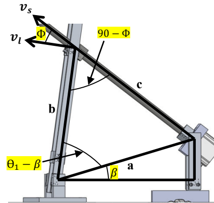
Fig. 4 Working triangle of first joint
