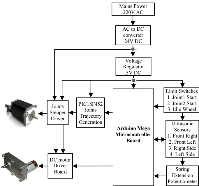
Fig. 18 Control architecture
