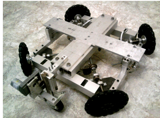
Fig. 17 Photograph of the mobile platform
