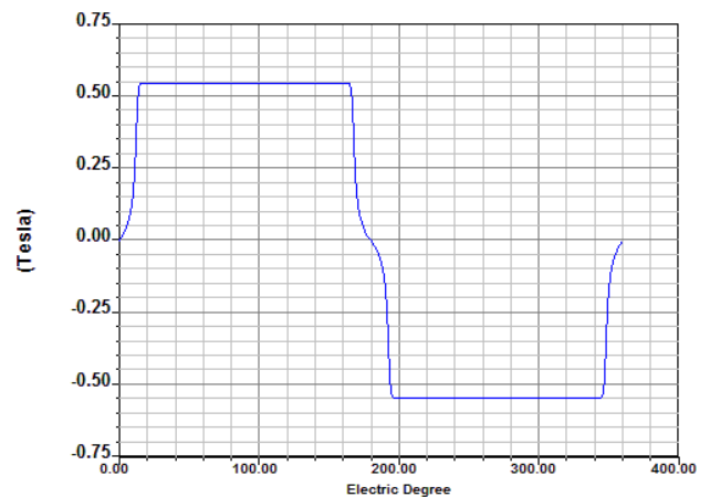
Fig. 18 Air gap flux versus electrical degree
