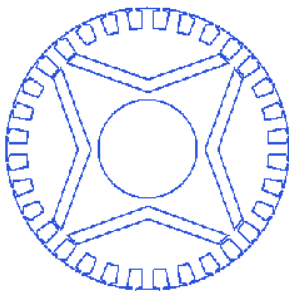
Fig. 15 Rotor structure of LSPMM at third state
