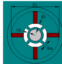
Fig. 5 Pole structure of LSPMM at first state
