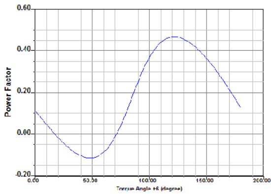
Fig. 7 Power factor versus torque angle
