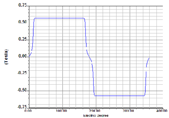
Fig. 12 Air gap flux versus electrical degree
