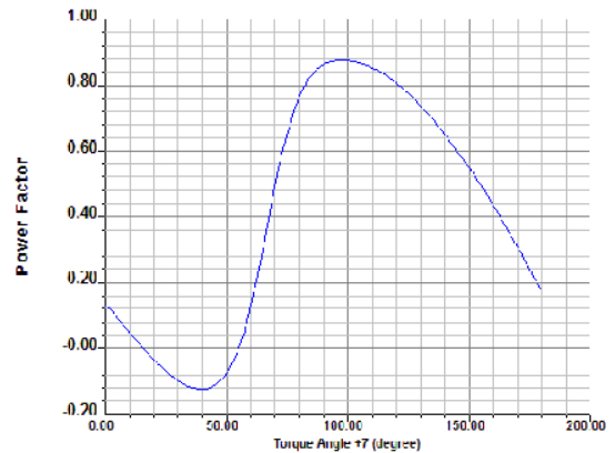
Fig. 13 Power factor versus torque angle
