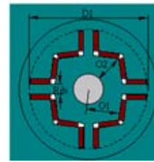
Fig. 10 Rotor structure of LSPMM at second state
