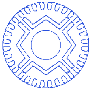
Fig. 9 Rotor structure of LSPMM at second state
