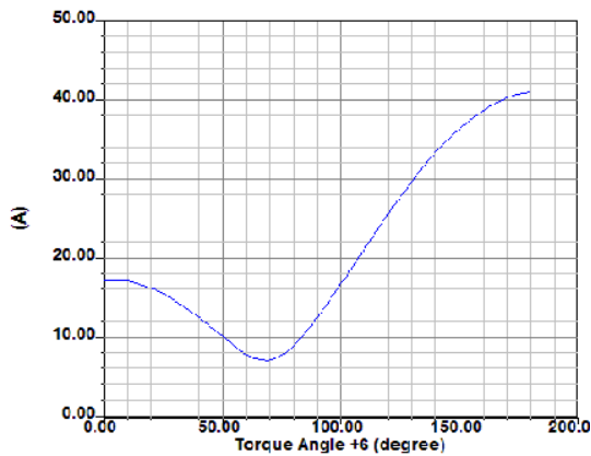
Fig. 14 Line current versus torque angle
