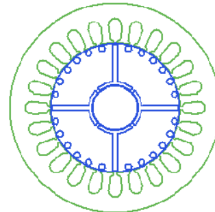
Fig. 6a LSPMM at first state
