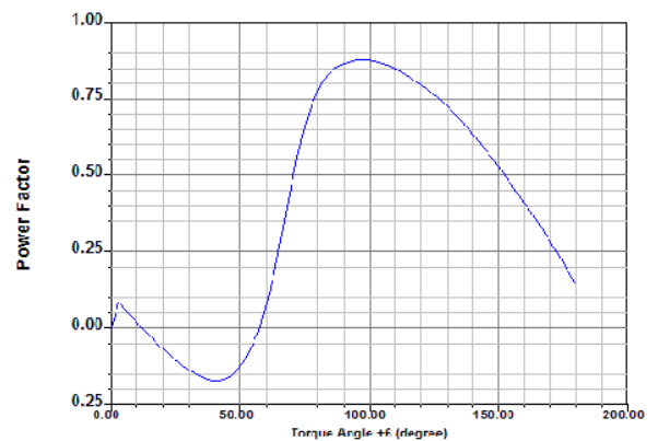
Fig. 19 Power factor versus torque angle
