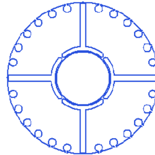
Fig. 4 Rotor structure of LSPMM at first state
