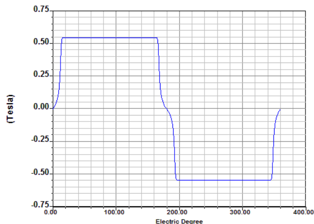
Fig. 18 Air gap flux versus electrical degree
