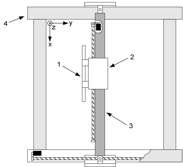
Fig. 3 Top view of the studied machine
