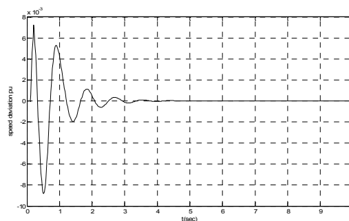
Fig. 7 Speed deviation for operating condition 2
