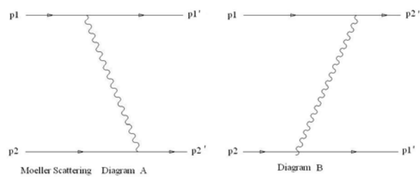
Fig. 14. Diagrams for Moeller Scattering
