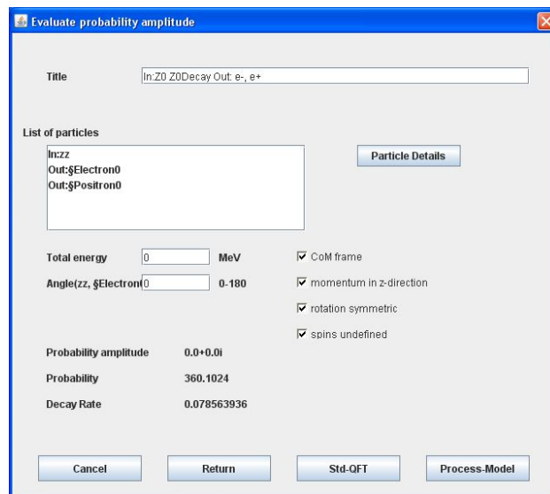
Fig. 17. Evaluation of |M|^2 and Decay Rate for Z0-Decay
