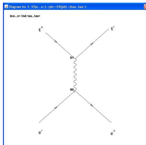
Fig. 8. Feynman diagram for the tauon pair creation e^-e^+ \rightarrow \tau^-\tau^+
