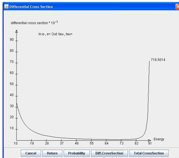
Fig. 11. Differential cross section for tauon pair creation, including weak interaction
