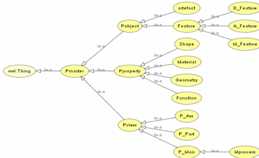
Fig. 1 Concept hierarchy of the product ontology
