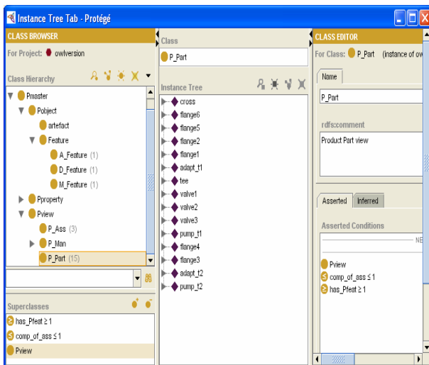
Fig. 4 Vacuum suitcase implementation in Protégé-OWL
