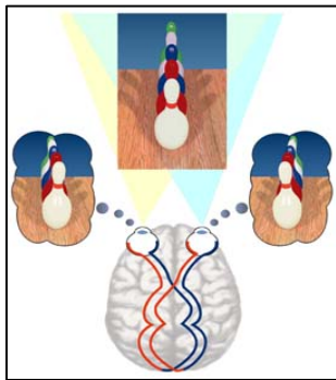
Fig. 2 Binocular Vision
