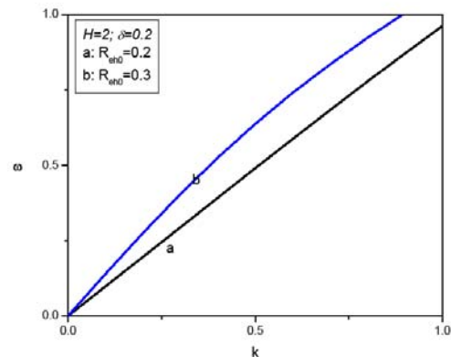
Fig. 1(a) Dispersion curves for different values of the relativity parameter R_{eh0} keeping \delta and H constant
