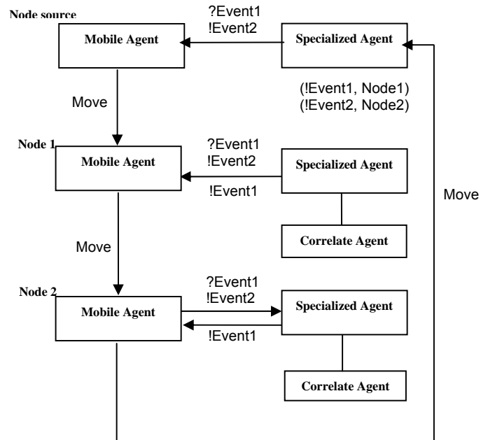
Fig. 2 Itinerary Example of a Mobile Agent
