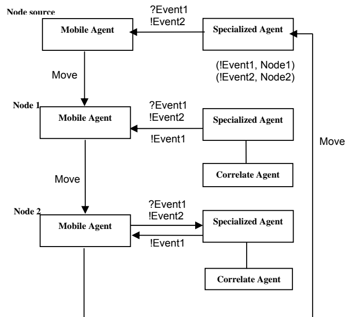
Fig. 2 Itinerary Example of a Mobile Agent
