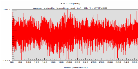
Fig. 4 Replicated stub axle load-time history
