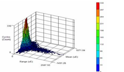
Fig. 5 Rainflow cycle matrix for the stub axle loads
