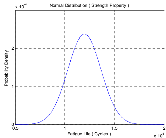
Fig. 8 Probability density function of stub axle
