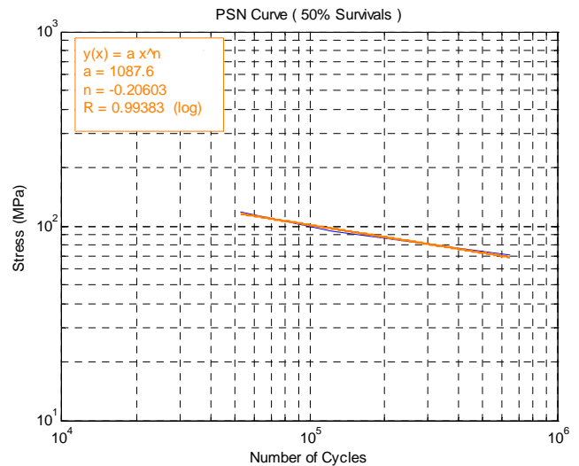
Fig. 7 Mean life probabilistic SN curve
